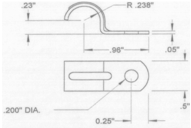
One Hole Strap 3/8" (Peco Part Numbers P38BX and P38BJ) For Use With 14/2, 14/3, & 12/2 Solid MC Cable
