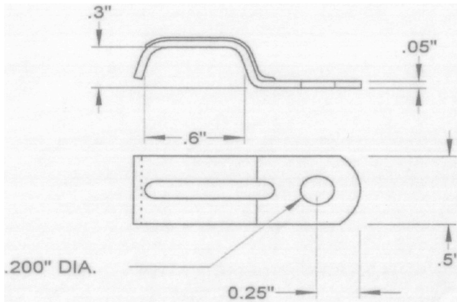
One Hole Non-Metallic Cable Strap (Peco Part Number P713J)
